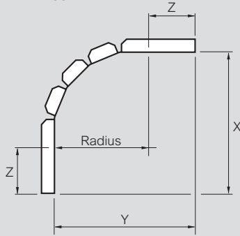
90° outside riser
