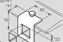
Window beam clamp SC852/41
